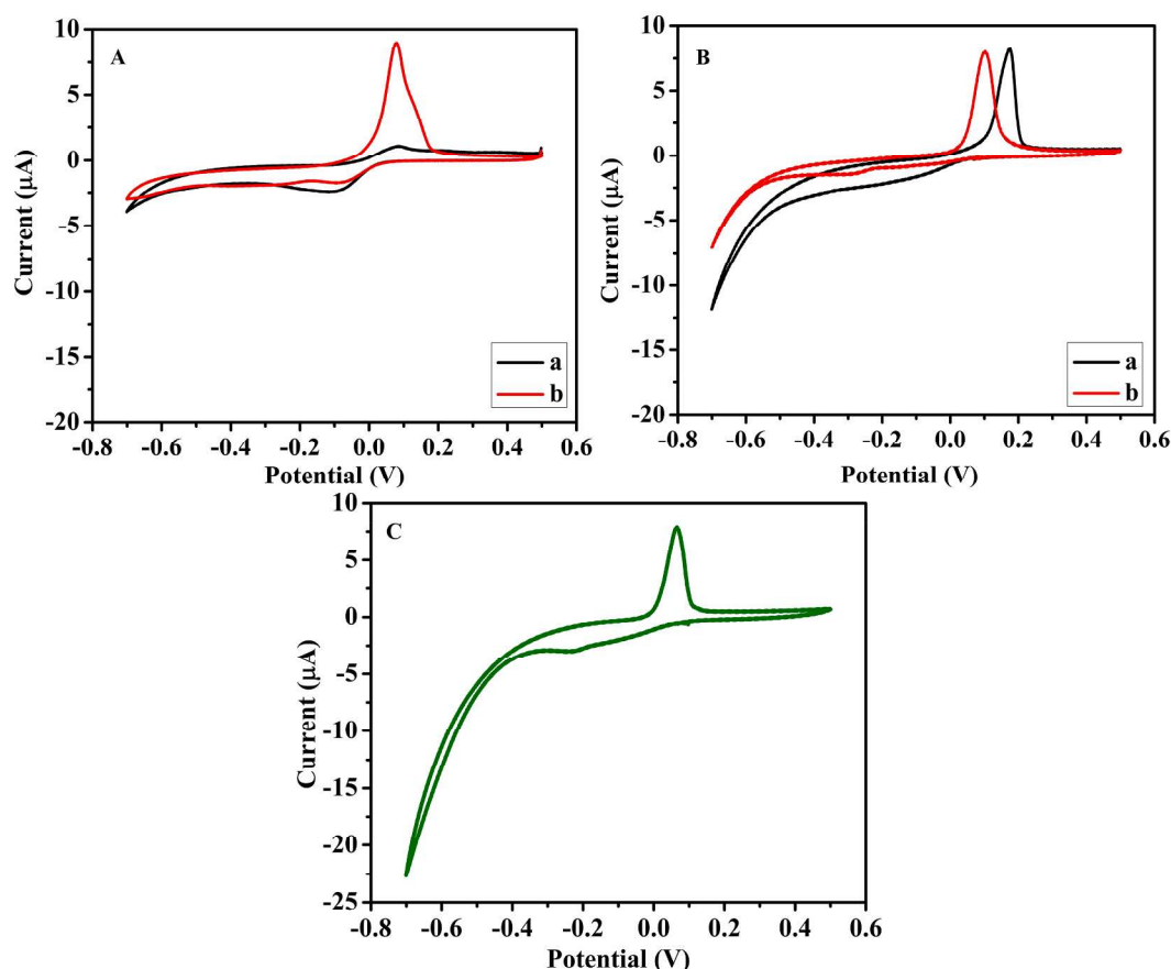
Fig. 1. (A) Cyclic voltammograms of 2 \times 10^{-4} \text{ mol L}^{-1} \text{ Cu}^{2+} in supporting electrolyte of 0.1 M \text{KNO}_3 in the presence of \text{O}_2 (a) and after degassing the solution (b). (B) Cyclic voltammograms of 2 \times 10^{-4} \text{ mol L}^{-1} \text{ Cu}^{2+} in the supporting electrolyte of 0.1 M \text{KNO}_3 containing 1 % PAA in the presence of \text{O}_2 (a) and after degassing of the solution (b). (C) Cyclic voltammograms of 2 \times 10^{-4} \text{ mol L}^{-1} \text{ Cu}^{2+} in the supporting electrolyte of 0.1 M \text{KNO}_3 and 1 % PAA in the presence of 2 \times 10^{-3} \text{ mol L}^{-1} \text{ H}_2\text{O}_2 in presence of \text{O}_2 . The scan rate for all voltammograms is 50 \text{ mV s}^{-1} .
