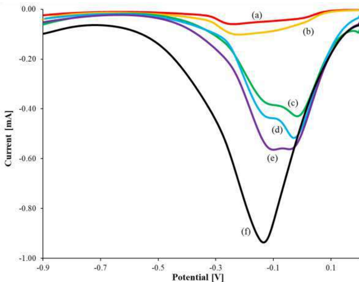
Fig. S3 SW voltammograms recorded at a Prussian blue screen printed electrode in 0.1 M KNO 3 and 1% PAA as the supporting electrolyte (a, d), in the presence of 2 \times 10^{-4} mol L -1 Cu 2+ (b, c, e, f) and increasing concentration of H 2 O 2 : (c) 0.5, (d, e) 1, and (f) 8 mM. SW parameters: frequency 8 Hz, SW amplitude 0.2 V, step potential -0.005 V.
