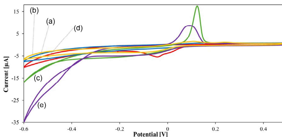
FIGURE 1 | Cyclic voltammograms recorded at a GCE, scan rate 50 \text{ mV s}^{-1} in selected supporting electrolytes: (a) 0.1 \text{ mol L}^{-1} \text{ KNO}_3 , (b) pAAmAA, (c) PAA, (d) pAMPS, and (e) neutralized pAMPS (pH 7). Each polyelectrolyte was 1% (w/v), all studied solutions were prepared in 0.1 \text{ mol L}^{-1} \text{ KNO}_3 with 1 \text{ mM} hydrogen peroxide and 2 \times 10^{-4} \text{ mol L}^{-1} copper ions(II).
