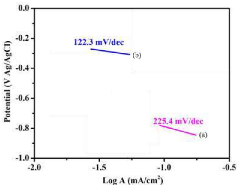
Fig. S1 Calculated Tafel slopes derived from linear sweep voltammetry (LSV) measurements (scan rate: 5 \text{ mV s}^{-1} ) recorded at bare screen-printed electrode for (a) 1% PAA with \text{H}_2\text{O}_2 (1 mM) and (b) 1% PAA with \text{Cu}^{2+} ( 2 \times 10^{-4} \text{ mol L}^{-1} ) and \text{H}_2\text{O}_2 (1 mM). Each solution contained 0.1 M \text{KNO}_3 .
