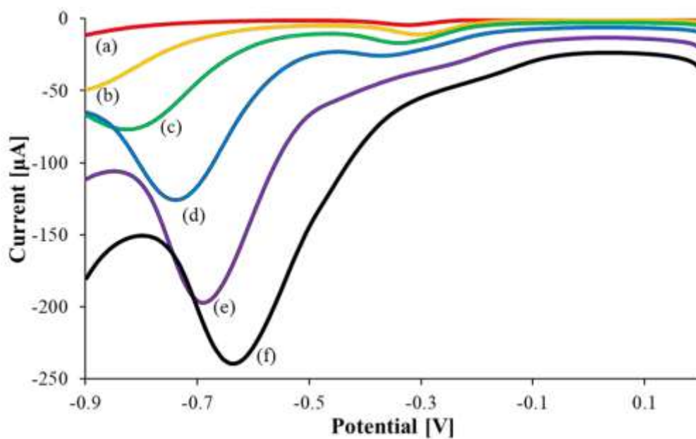
Fig. S3 SW voltammograms recorded at a Prussian blue screen printed electrode in 0.1 M KNO 3 and 1% PAA as the supporting electrolyte (a, d), in the presence of 2 \times 10^{-4} mol L -1 Cu 2+ (b, c, e, f) and increasing concentration of H 2 O 2 : (c) 0.5, (d, e) 1, and (f) 8 mM. SW parameters: frequency 8 Hz, SW amplitude 0.2 V, step potential -0.005 V.
