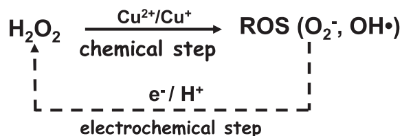
Scheme 1. The assumed reaction pathway for the electrocatalytic mechanism of a second kind giving rise to the reduction current tail at potentials more negative than -0.400 \text{ V} .
